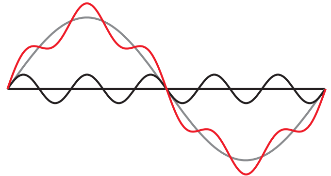
The total current as the sum of the fundamental and 5 th harmonics
